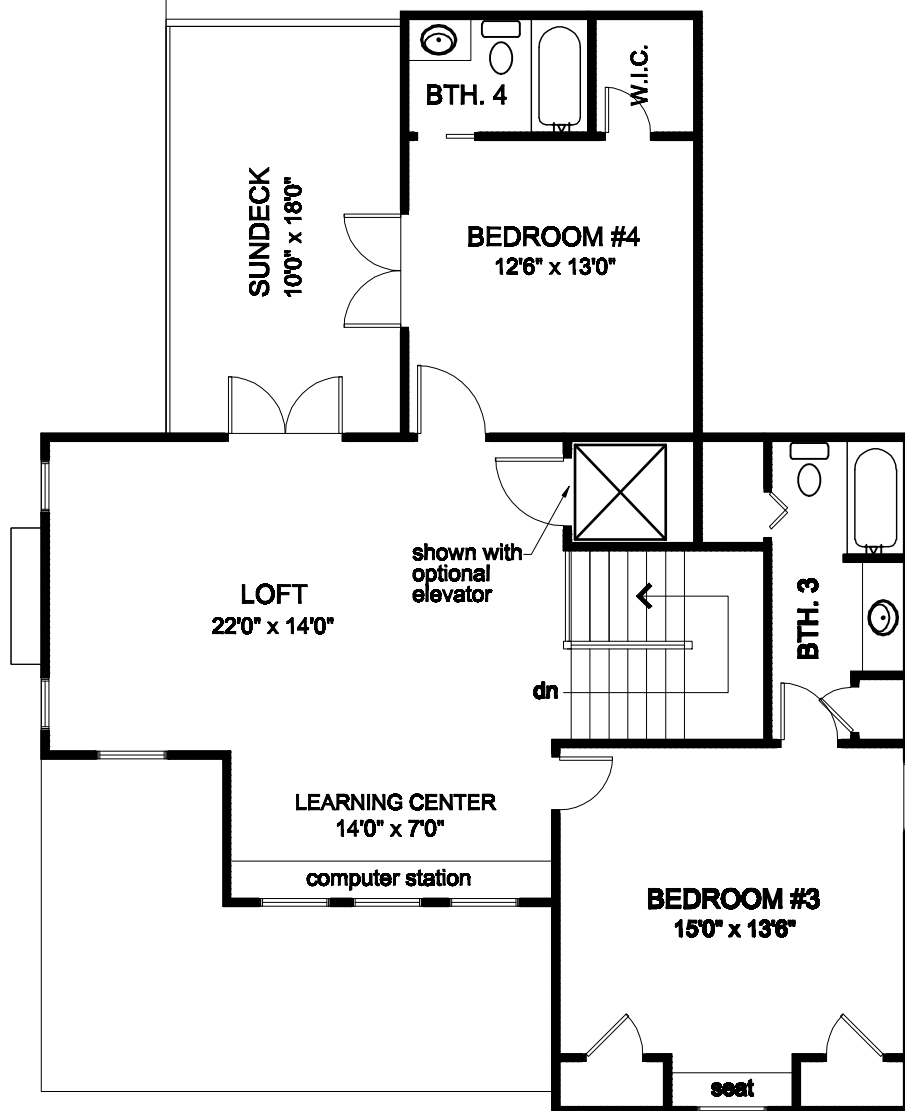
2nd FLOOR PLAN "b"
